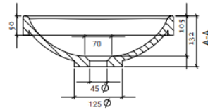
Side Section
