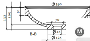
Side Section
