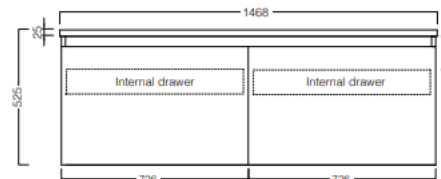
Front On
