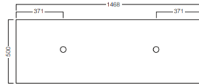
Top Down
