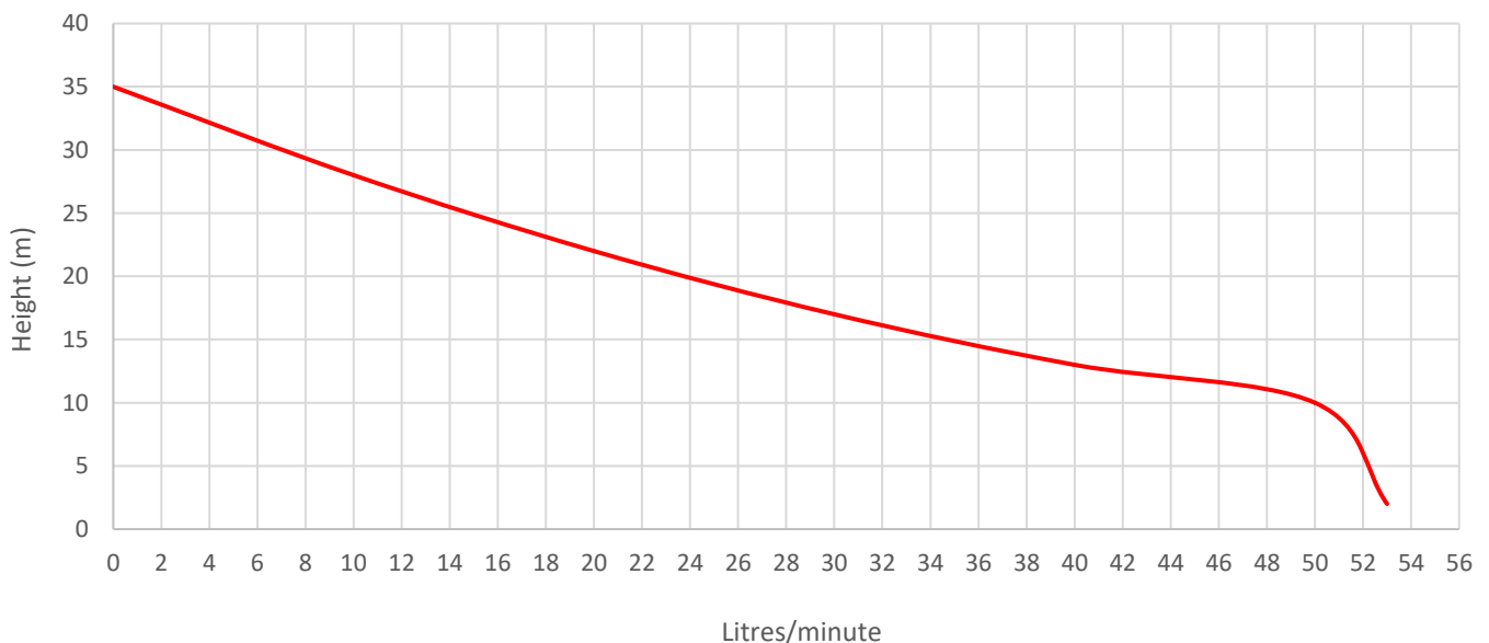
Pump Performance
